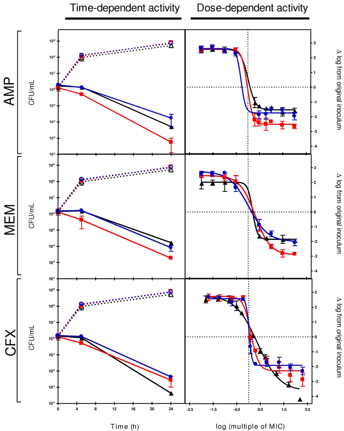
Figure 1 Activities of ampicillin (AMP), meropenem (MEM) and cefuroxime (CFX,) were tested against EGDe wild-type (triangle), \Delta PBP4 (squares) and \Delta Lmo0441 (circle). Left panel shows bacterial growth (open symbols, discontinuous lines) and antibiotic activity (closed symbols and continuous lines) during 24h at 100 times MIC in TSB broth. Right panel shows, at 24h, the dose response curves of the 3 same antibiotics in TSB broth. Curve fitting and statistical analyses were performed using GraphPad Prism for windows version 4.03 and GraphPad InStat version 3.01 (GraphPad® Software, San Diego, CA).
